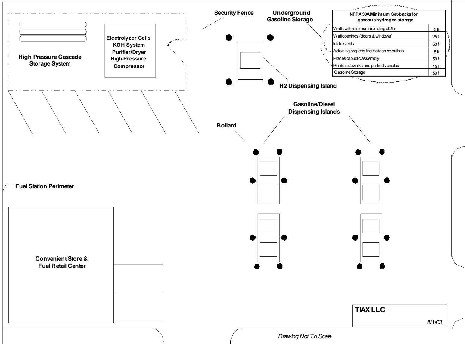
Figure 4-8. Electrolyzer-Based Refueling Station Site Plan
