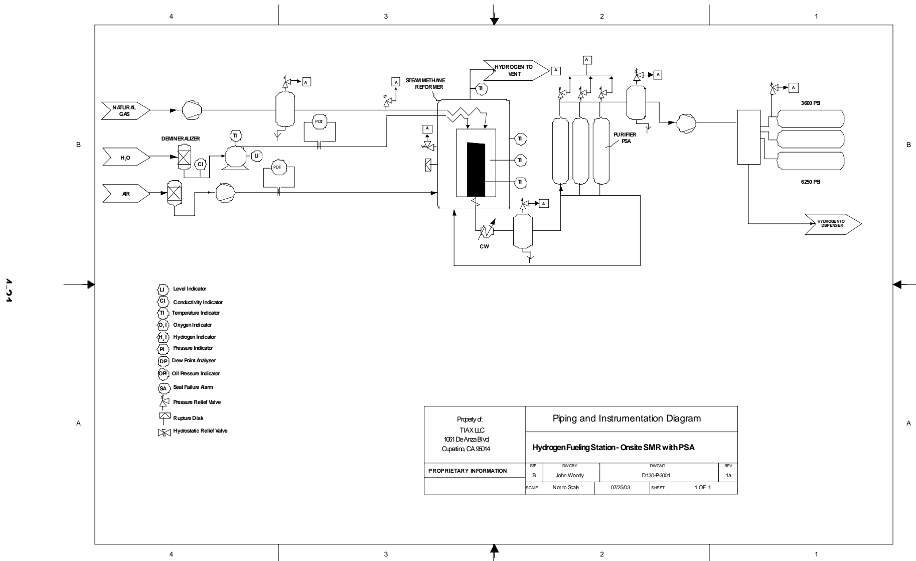
Figure 4-10. Piping and Instrumentation Diagram for Steam Methane Reforming-Based Refueling
