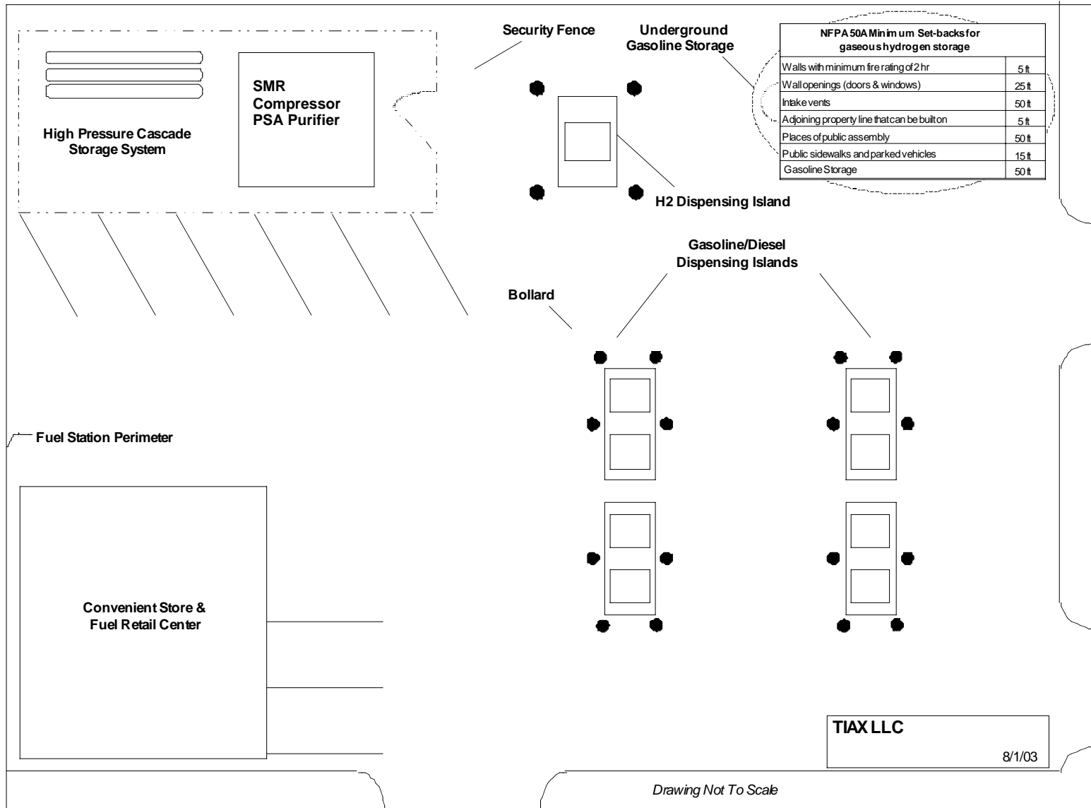
Figure 4-11. SMR-Based Refueling Station Site Plan
