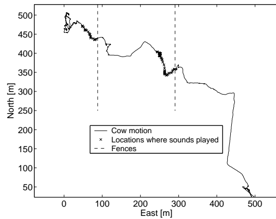
Figure 16: Trace of the position of cow #10 during an experiment with two virtual fences. The cow started in the barn, at the SE corner of the plot. Locations where sounds were played automatically are shown. The long straight line to the north is the walk from the barn to the field, which is not considered in our analysis. After the first fence (to the east) timed out, no sounds played until a second fence (to the west) was created.
