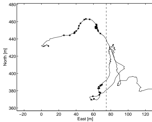
Figure 17: Trace of the position of cow #9 during the virtual fence experiment. A small portion of the experiment is shown, during which the cow walked past the fence on two separate occasions, showing correct behavior of the virtual fence algorithm.
