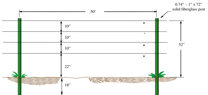
Figure 8. 4-wire electric fence.
